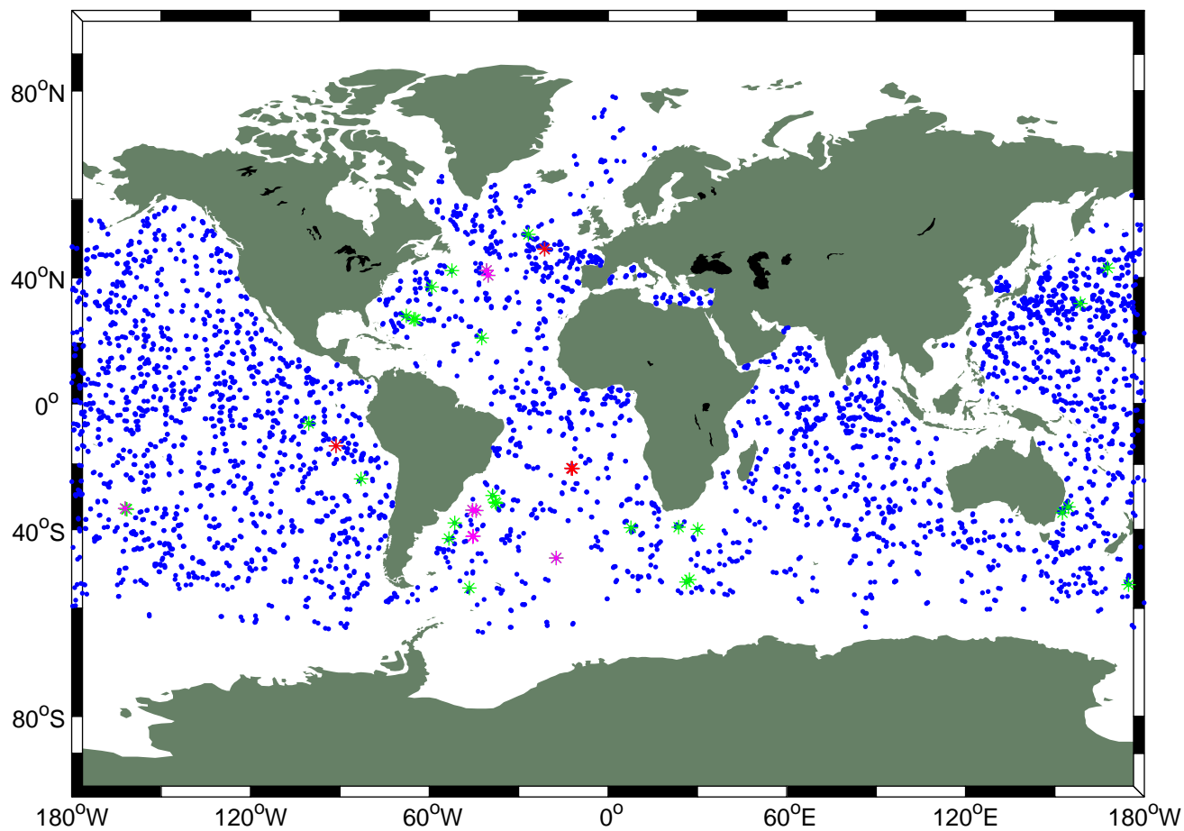
Anomalies Psal. ARGO / std lev green points >3std ;magenta points >5std ; red points >10 std
